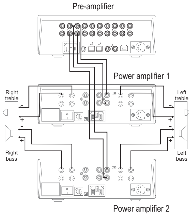
Connecting a bi-amplified speaker system to a pre-amplifier
