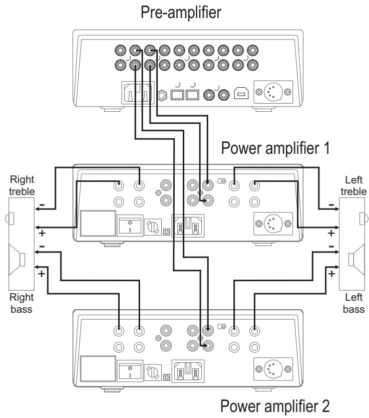
Connecting a bi-amplified speaker system to a pre-amplifier
